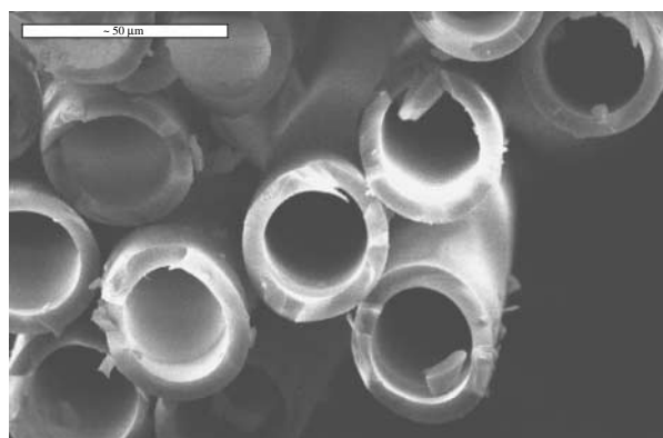
Figure 2. Typical hollow glass fibre (35 µm external diameter with 55% hollowness fraction).
